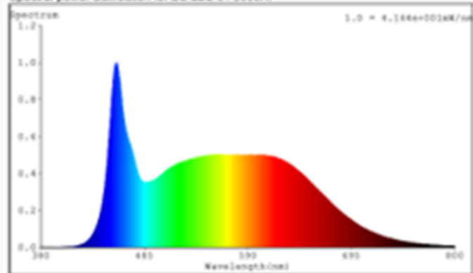
Spectral power distribution for DL-LDL-01 5000K:
